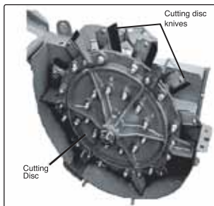
Cutting Unit:
